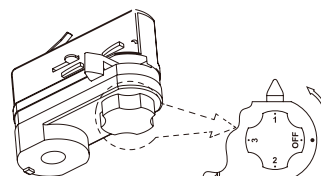
4-wires adaptor
