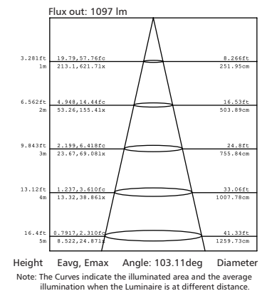
Beam diagram
